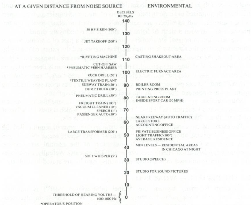
Figure 2-1. Typical A-weighted sound levels measured with a sound-level meter. These values are taken from the literature. Sound-level measurements give only part of the information usually necessary to handle noise problems, and are often supplemented by analysis of the noise spectra.
