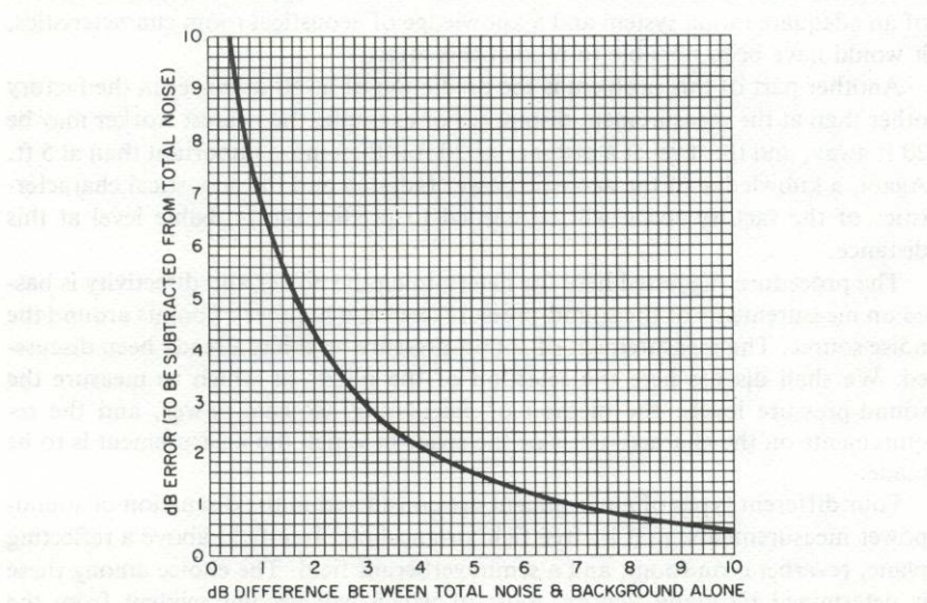
Figure 13-6. Background noise correction for sound-level measurements.
