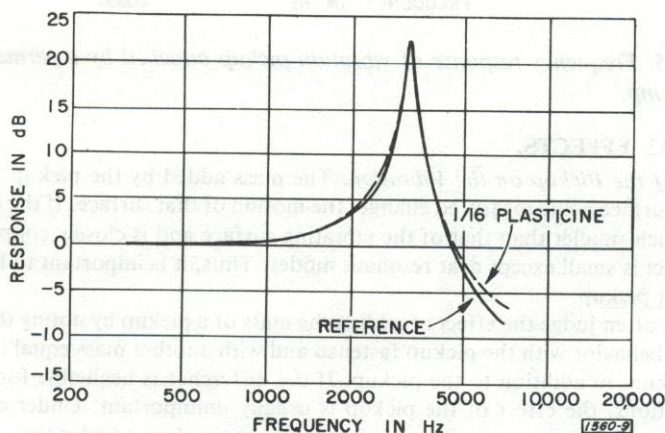
Figure 15-4. Frequency response of vibration pickup attached by means of 1/16-in. thick layer of plasticene.
