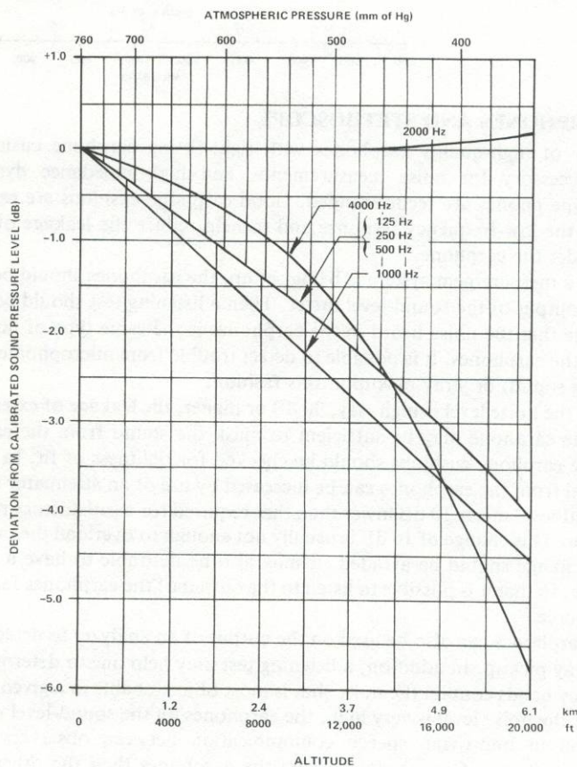
Figure 12-2. Change in output of the GR 1986 Omnical Sound-Level Calibrator as a function of atmospheric pressure.
