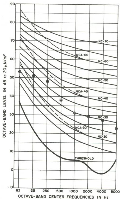
Figure 4-6. Noise-criteria curves.
