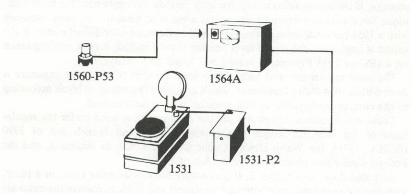
Figure 11-9. Tenth octave-band vibration analysis with stroboscopic observation.
