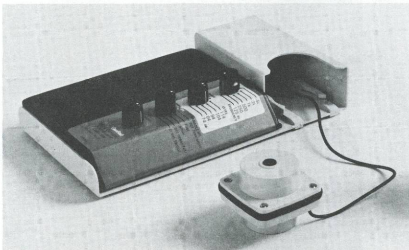
Figure 7-5. 1986 Omnicul Sound-Level Calibrator.
