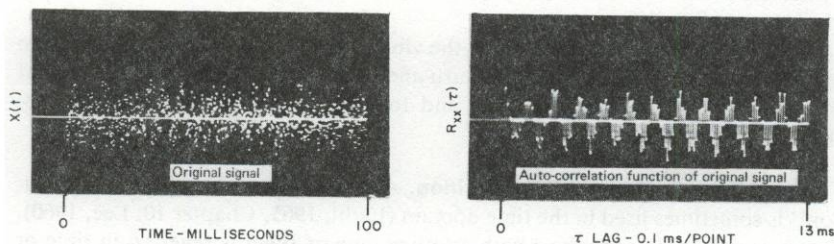
Figure 8-8. Auto correlation analysis of sinewave buried in noise.
