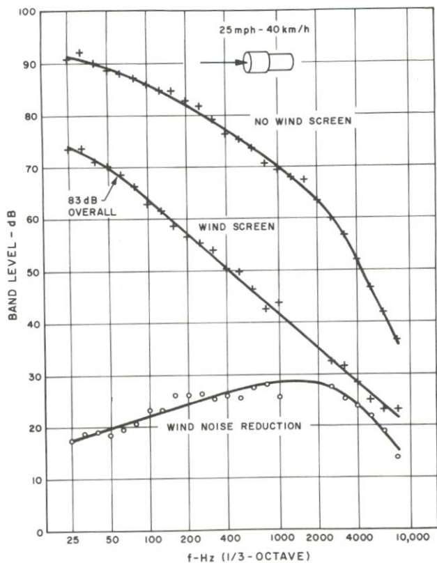
Figure 6-13a. Wind-noise spectrum, flat weighting.
