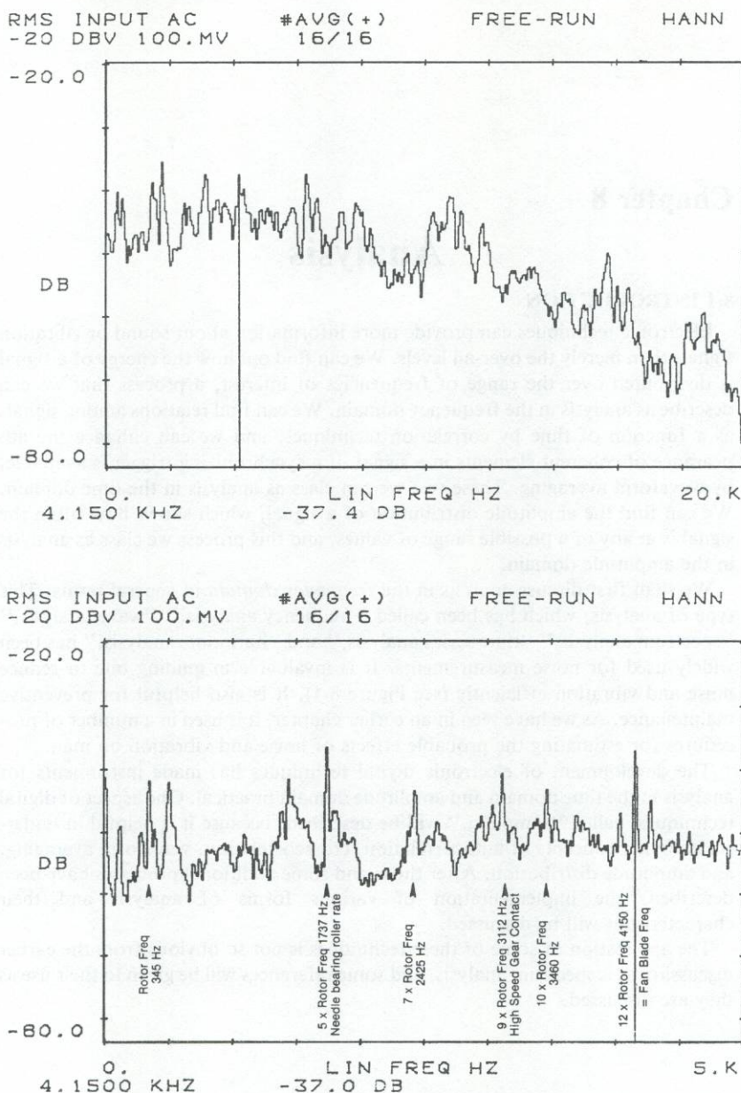
Figure 8-1. Chart records of the sound spectrum of a motor and gear-train assembly (see sketch). Both records were taken on a Type 2512 Spectrum Analyzer. The 20-kHz range shows the full audible spectrum with significant components extending out to beyond 10 kHz. The 5-kHz range shows more detail for the region of greatest concern for quieting. Most of the important components are simple multiples of the high-speed rotor frequency.
